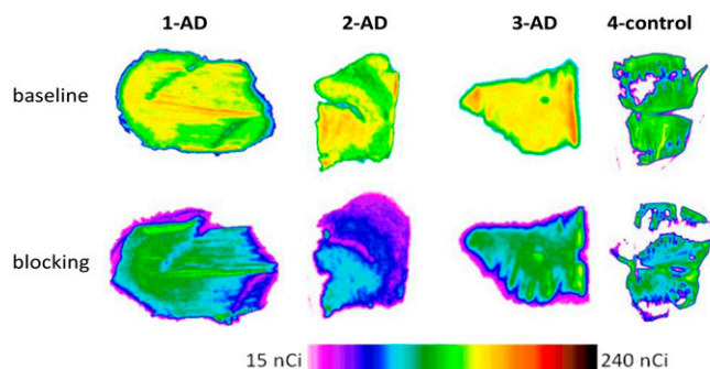
Fig. 6. Postmortem human autoradiography/[ ^{11}\text{C} ]CPPC images (baseline and blocking) in inferior parietal lobe gray matter slices. Three subjects with Alzheimer's disease (1-AD, 2-AD, and 3-AD) and control (4-control) subject. See also SI Appendix, Fig. S14 and Tables S5 and S6 .
