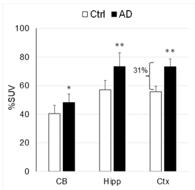
Fig. 3. Comparison of the [^{11}\text{C}]\text{CPPC} brain uptake in transgenic AD ( n = 6 ) and control ( n = 5 ) mice. Time-point – 45 min after radiotracer injection. Data: mean \% \text{SUV} \pm \text{SD} . * P = 0.04 , ** P < 0.005 (ANOVA). The uptake of [^{11}\text{C}]\text{CPPC} was significantly greater in AD mouse brain regions. CB, cerebellum; Ctx, cortex; Hipp, hippocampus.
